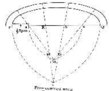
Five centered arch
