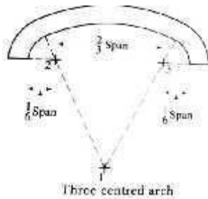
Three centered arch
