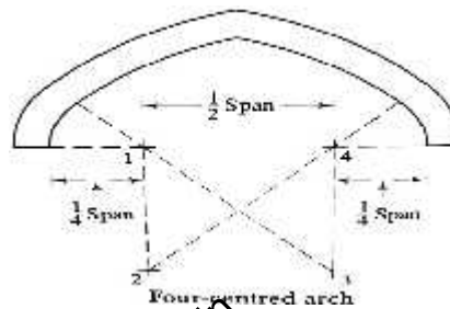
Four centered arch
